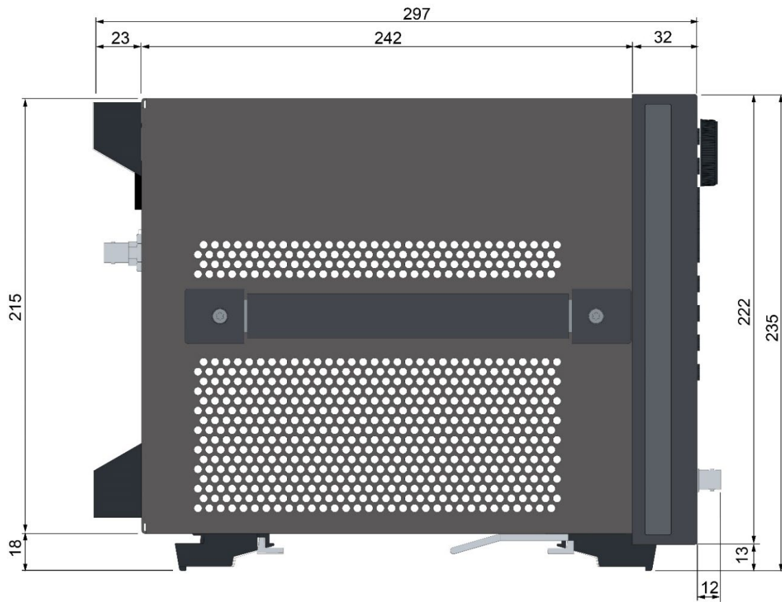
Figure 12. Side view (Millimeters)
